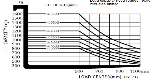
CAPACITY CHART
